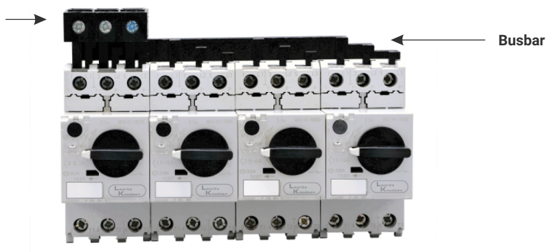
4 MMSs with busbar connection
