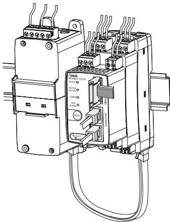
1. Side-wise mounting
