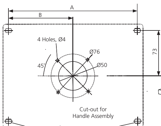
Switch Mounting Holes
