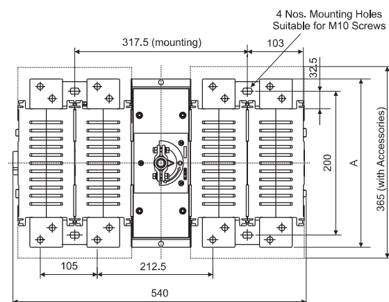
1000/1250 Terminal Arrangement
