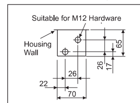
1600 Terminal Arrangement
