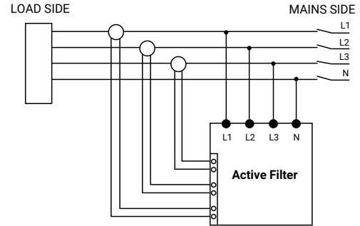
Open Loop Connection
