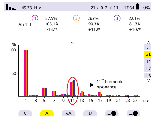
Figure 2: Measurement with APFC Panel ON
