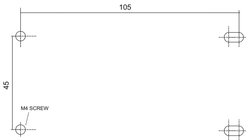
DRILLING PLAN FOR MO 50/60/70
